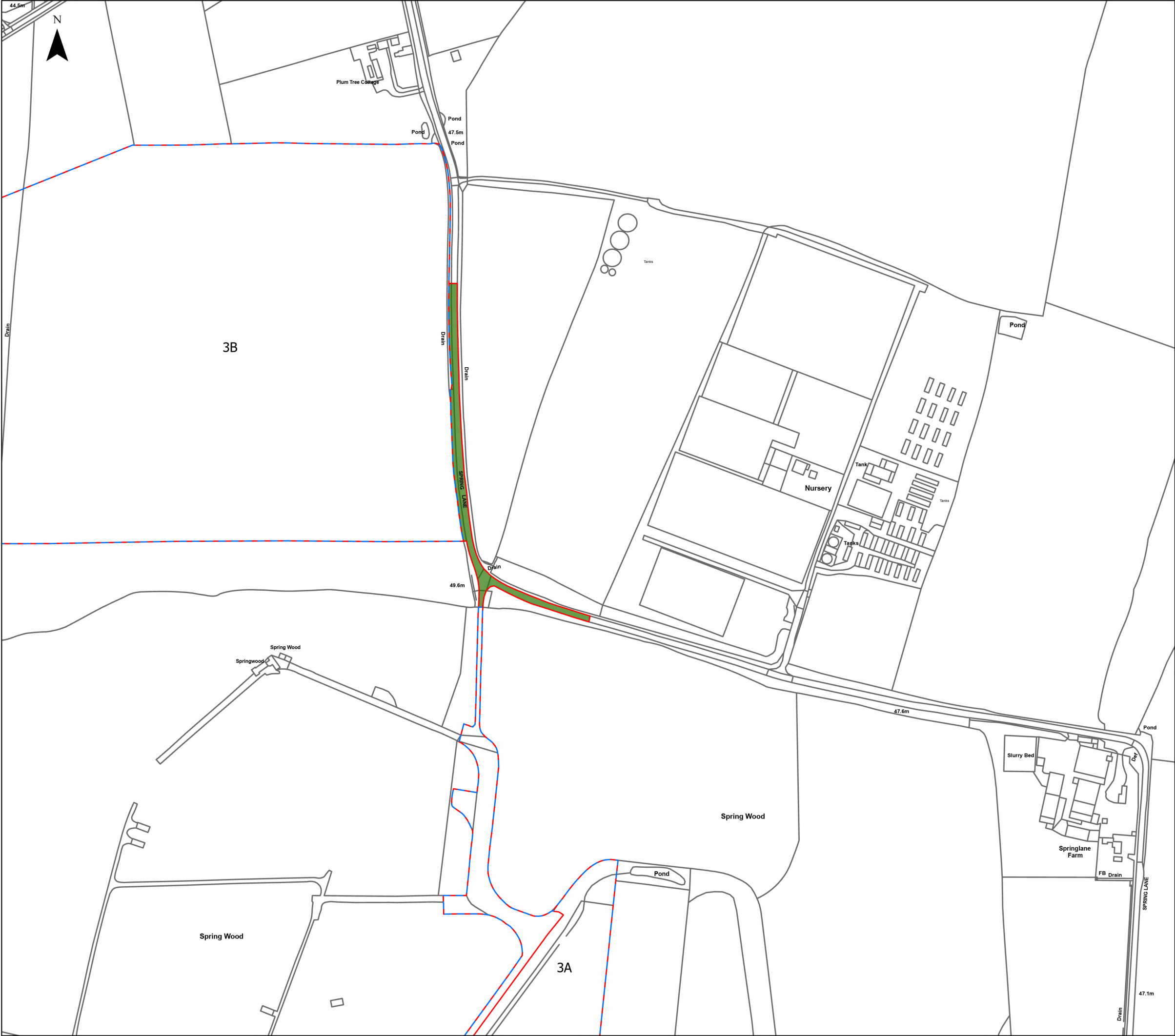
Figure 5.3: Alterations to the Site Boundary Between Scoping and PEIR Sheet 23 of 30 Revision B
